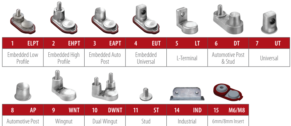
Figure 1 – Terminal Types
